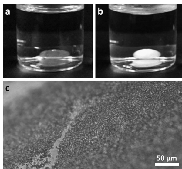
Figure 1. Photographs taken a) 15 s and b) 25 min after placing a large drop of chloroform containing 10 mg mL −1 of as received PS-PNIPAM into deionized water. c) Optical micrograph of the μm-scale w/o emulsion droplets spontaneously formed at the macroscopic o/w interface, which account for the increase in cloudiness seen from (a) and (b).
